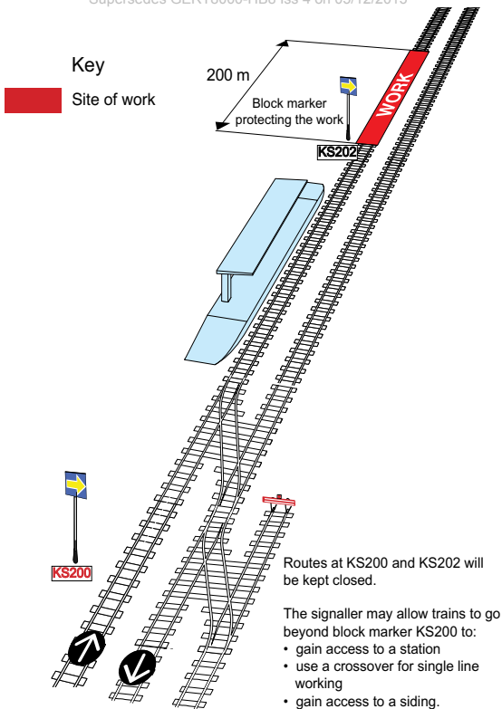
Diagram HB8-6 Work taking place close to the protecting block marker
