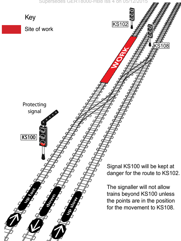
Diagram HB8-1 Work taking place beyond points that will be used
