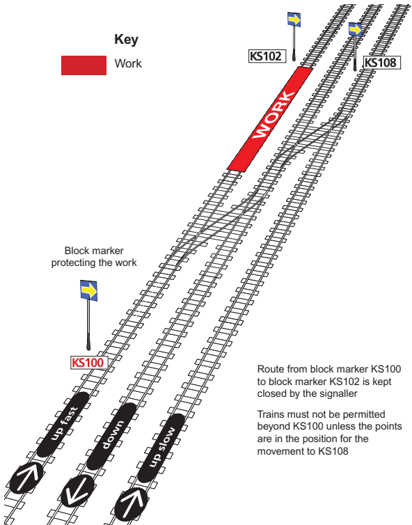
Diagram HB8-2 Work taking place beyond points that will be used
