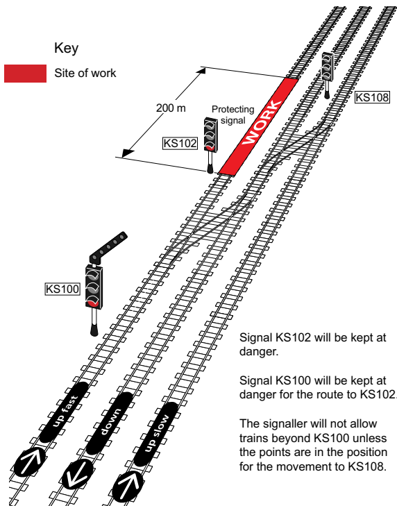
Diagram HB8-3 Work taking place close to the protecting signal
